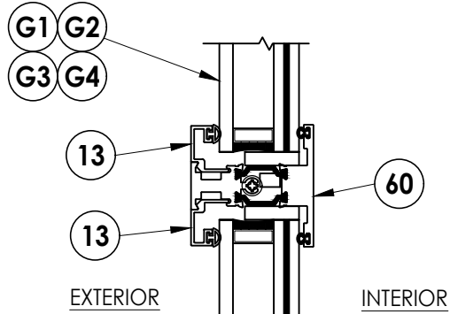
4 2 VERTICAL CROSS SECTION
