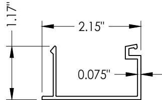
2 FRAME SNAP-IN
