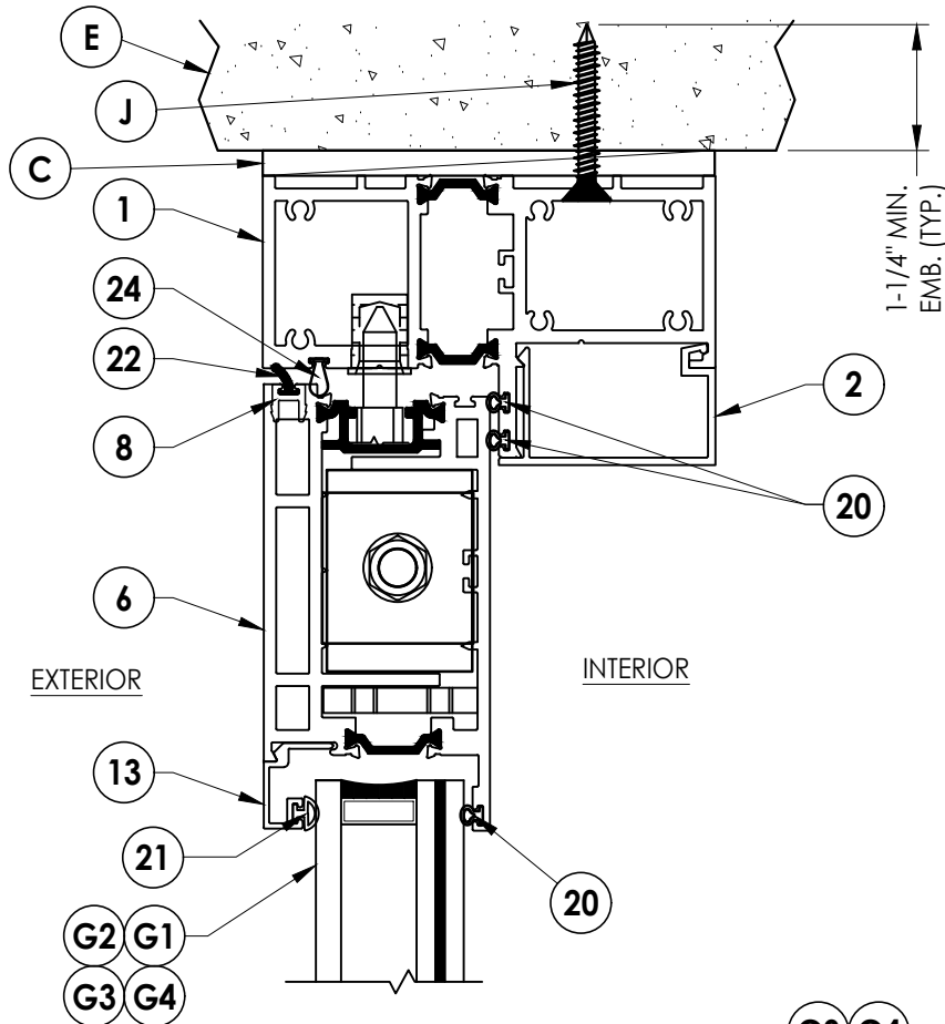
2 VERTICAL CROSS SECTION 6 Outswing Shown
