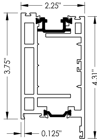
6 SASH
