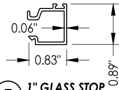
7 1" GLASS STOP
