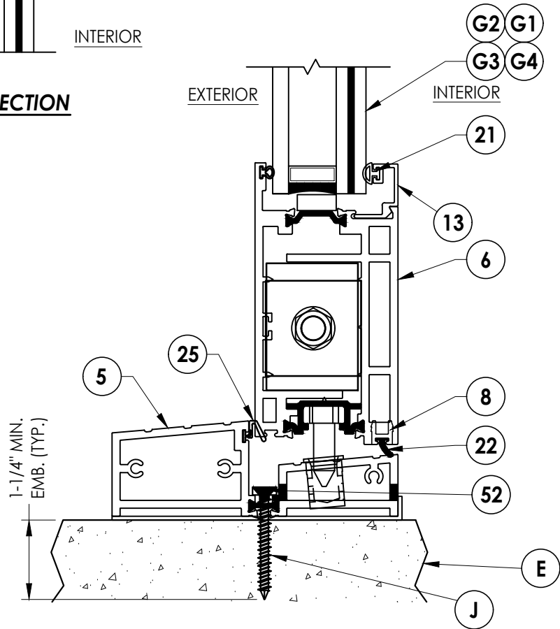
3 VERTICAL CROSS SECTION 6 Inswing Shown
